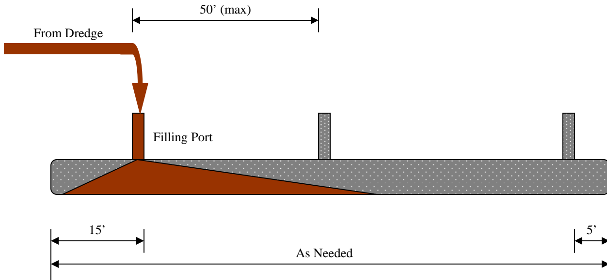
Dewatering Tube – 30' Circumference
