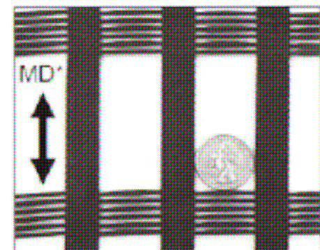
Aperture Size 1.00" x 0.63"
